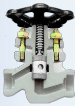
PISTON VALVE
